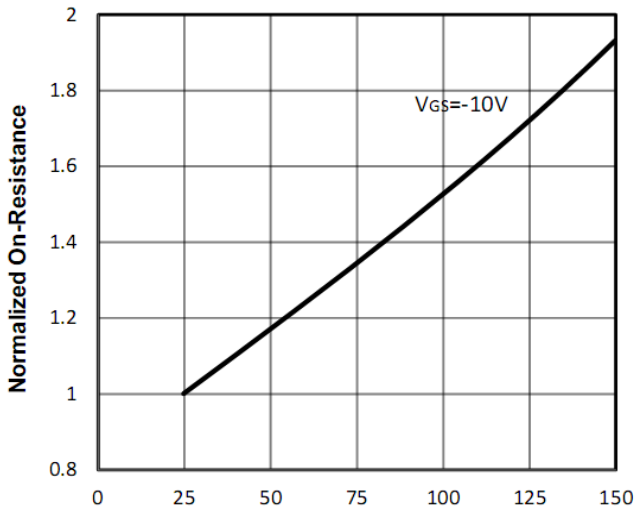
Figure13: -T J Junction Temperature (°C)
